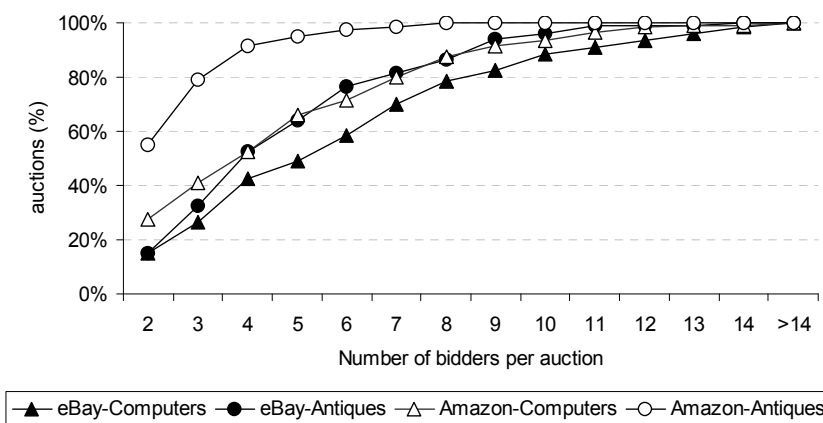
Figure 1. Cumulative distributions of numbers of bidders per auction
